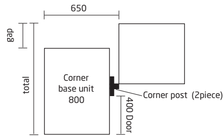
800mm Conventional Corner Base Unit
