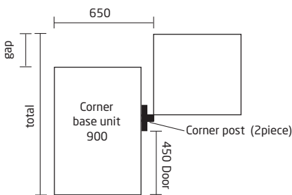
900mm Conventional Corner Base Unit
