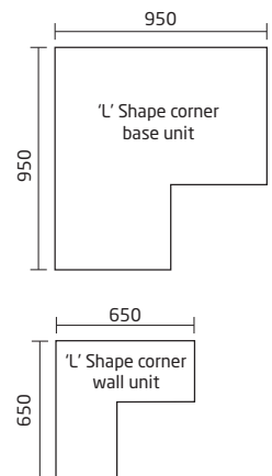
'L' Shape Corner Units Note:- Walls must be square to accommodate L shaped units.
